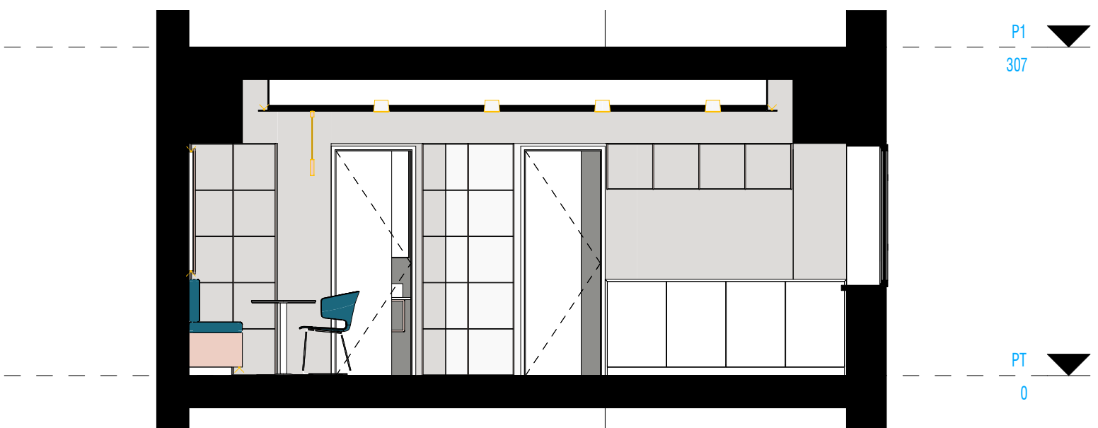
East Interior Elevation
