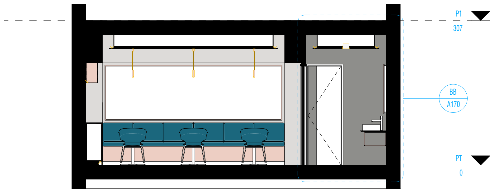
North Interior Elevation
